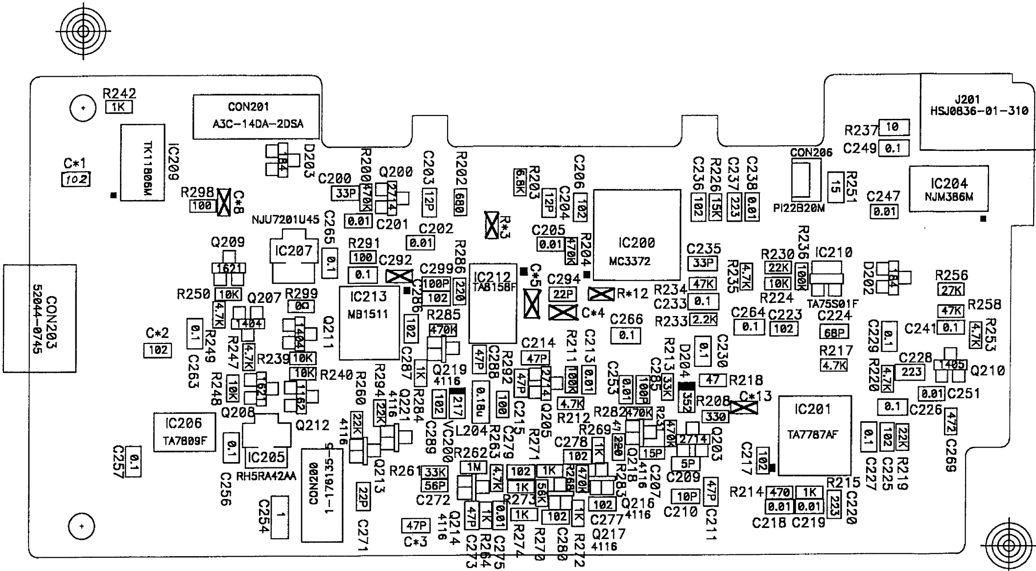
HSC-200 IF PCB BOTTOM VIEW (97/01/30)
